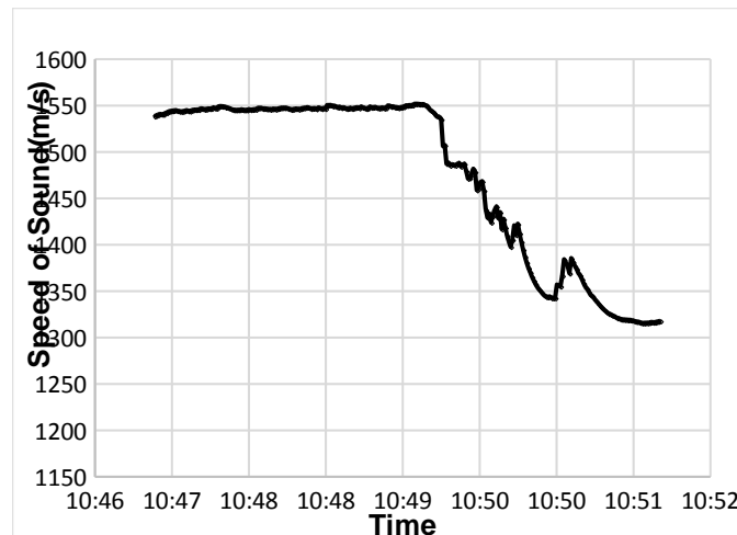
Figure(1) Passage of a Water/Oil Interface
